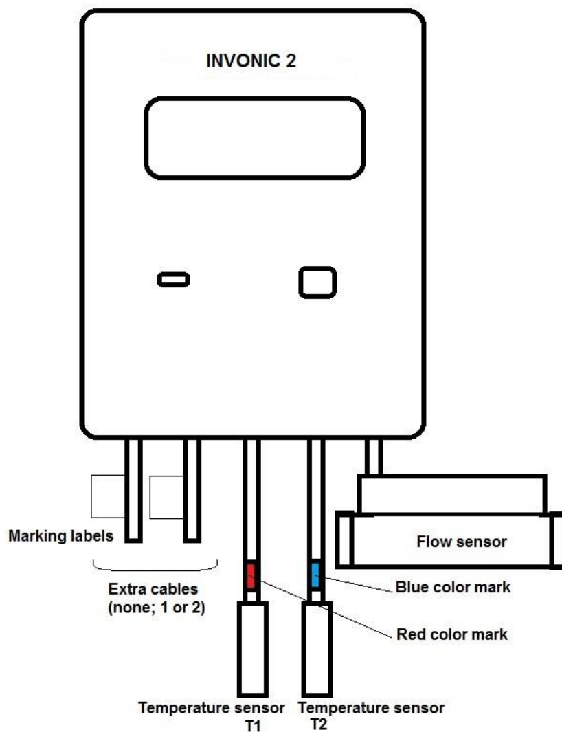
Fig. 5. Meter connection diagram
