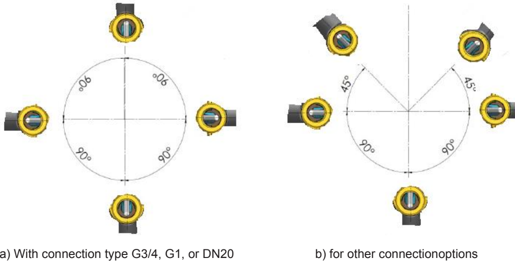
Fig. 2. Allowed installation positions of the flow sensor
