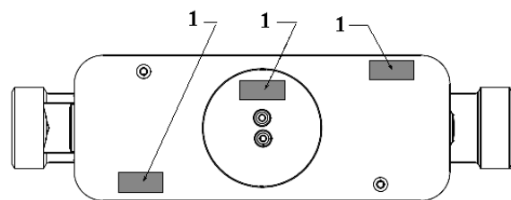
Fig. C1. The sealing diagram of calculator (at the back side of the box): It shall be sealed additionally only if the breakable partitions are damaged (1 – the supplier's seal is attached after installation; 2 – verification seal stickers are attached)
