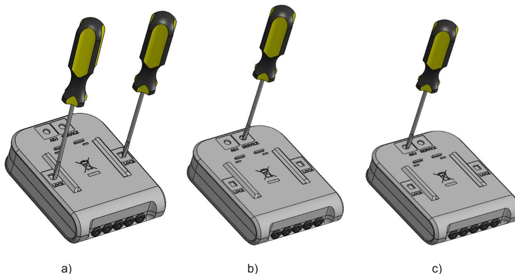
Fig. 1. Access to elements fixing the opening of the box (a), configuration change (b) activation contacts, and adjustment data change activation contacts (c) (partitions easily breakable with a tool)
