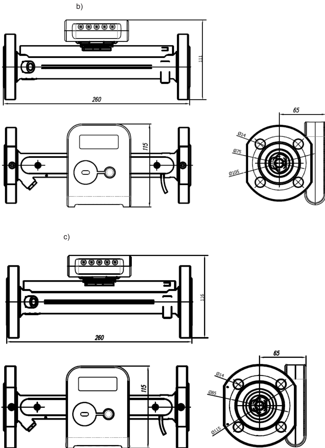
Fig. B2.4.. Flow sensor q_p = 3.5 \text{ m}^3/\text{h} ; L=260 \text{ mm} a) connection type: thread G11/4"; b) connection type: flanges DN25; c) connection type: flanges DN32
