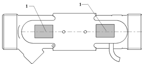
a) Flow sensor q_p = 0.6/1.0/1.5/2.5 \text{ m}^3/\text{h}
